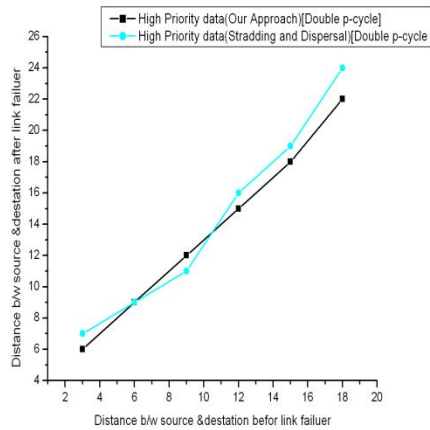
Figure.3(b) Higher Priority data Survivable Using Double p-cycle.
