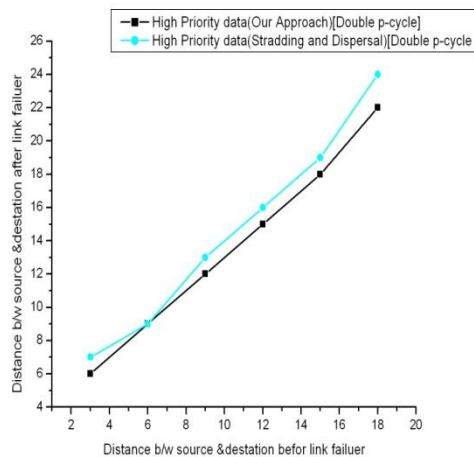
Fig: 3(d) on cycle and Straddle link Failure.
