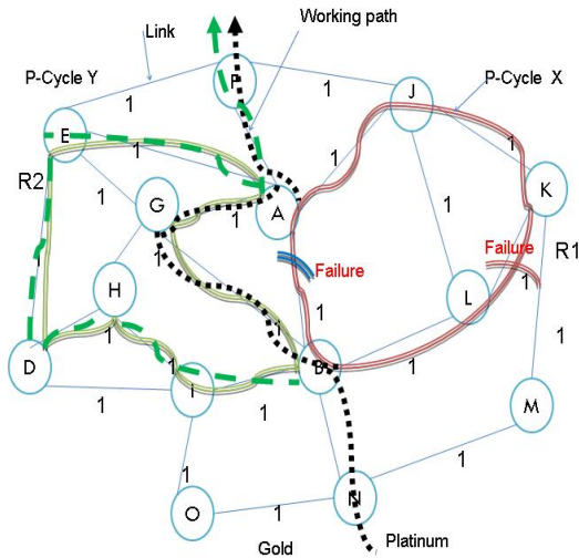
Figure.2 (c) Dual failures
