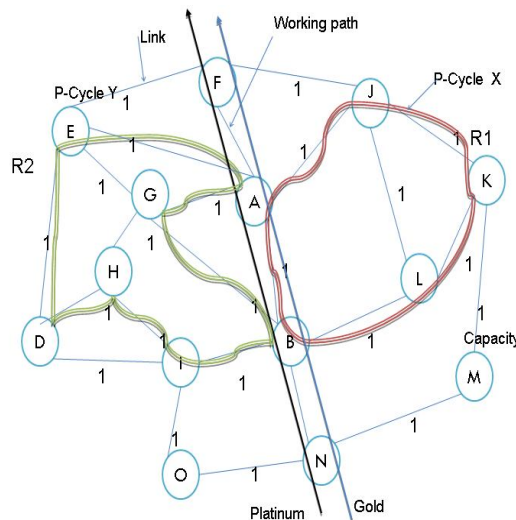
Figure.2(a) working Path of Double p-Cycle
