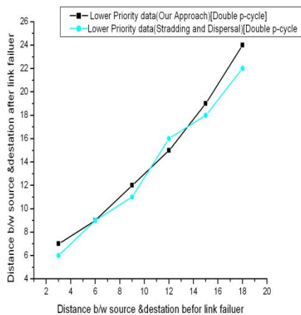
Figure.3(c) Lower Priority data Survivable Case II: On cycle and Straddle link failure in doubleP-cycle.
