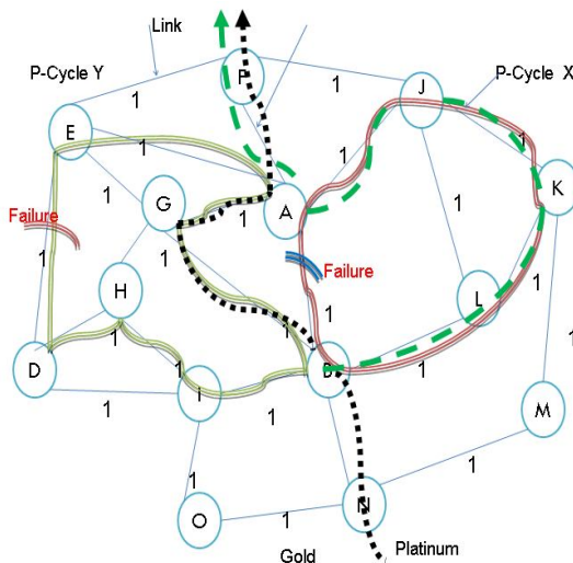
Figure.2 (d) Other Solution for data survivability.
